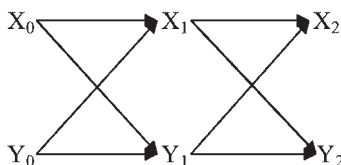
c. X and Y both measured on three occasions
