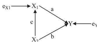
c. Control variable ( X_1 ) caused by substantive variable ( X_2 )
